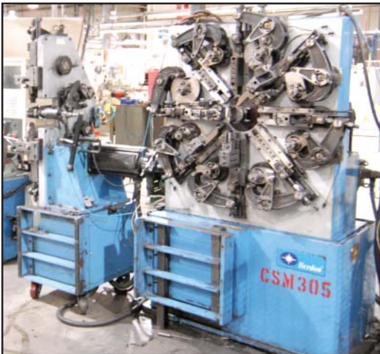
HERDON CSM 30T, CNC spring former
