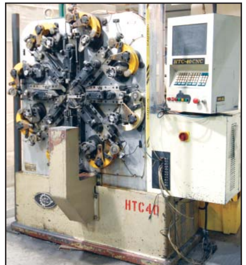
HTC 40 CNC, spring former
