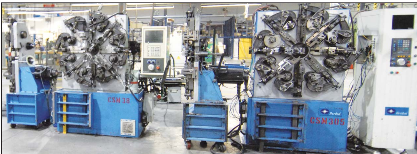
View of HERDON CSM 30, CNC spring machines
